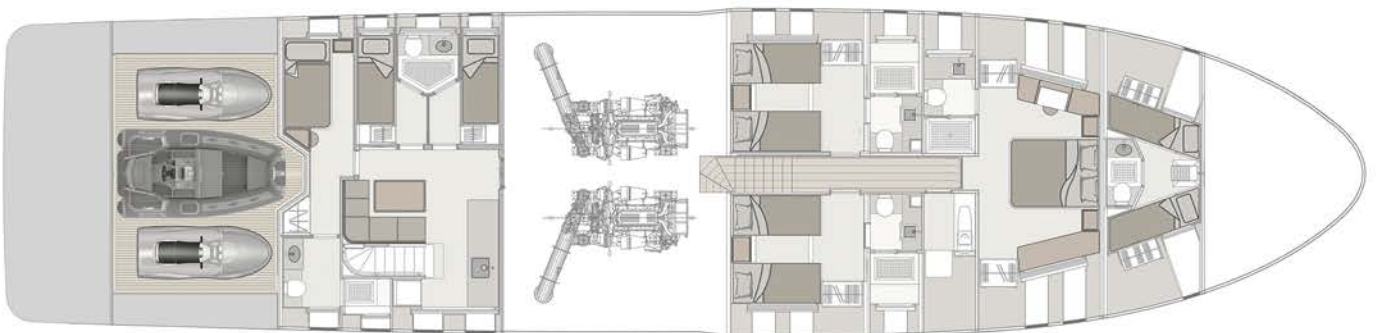
LOWER DECK
